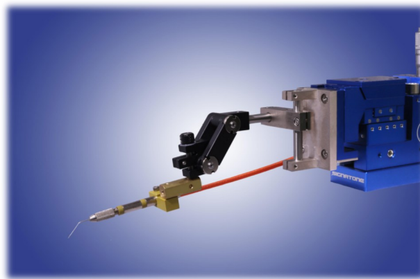
Figure 2 HVP-TX-3 mounted on a SP100 positioner
