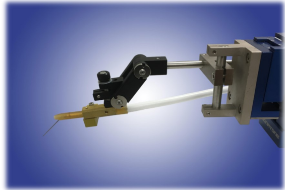
Figure 2 HVP-UX-20 mounted on a SP100 positioner
